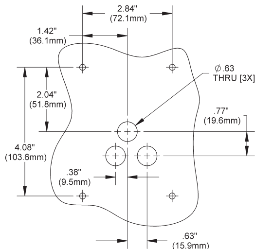
Fig 2: Mounting Hole Pattern
