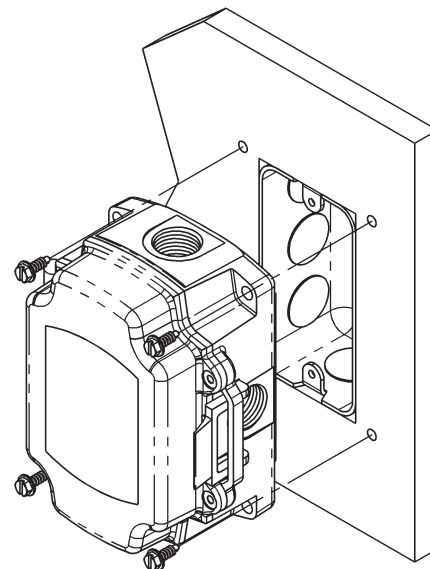
Fig 3: Mounting Screws Location
